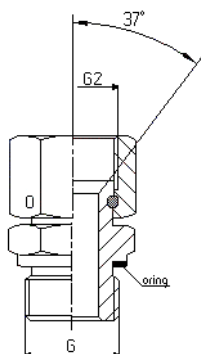
JIC EGE BSP / UNF
