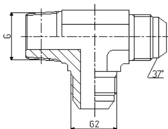
JIC XTEL BSPT / UNF JIC XTEL NPT / UNF
