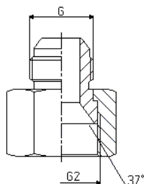
JIC RI UNF / UNF
