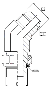
JIC 45 XWEP UNF / UNF
