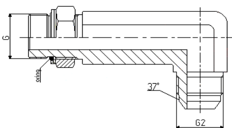
JIC XWESVGBSP / UNF
