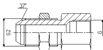
JIC XSVGW BSP / UNF JIC XSVGW NPT / UNF
