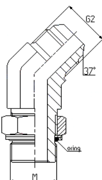
JIC 45 XWEP M / UNF
