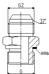
JIC XGE BSP / UNF
