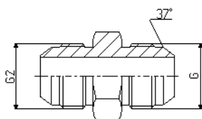
JIC XGR UNF / UNF
