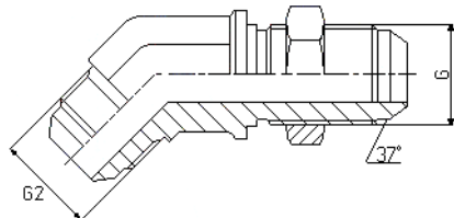
JIC XESV UNF / UNF
