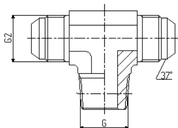
JIC XTET BSPT / UNF JIC XTET NPT / UNF
