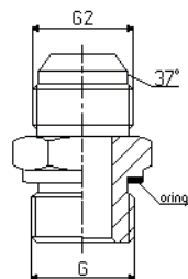
JIC XGE UNF / UNF
