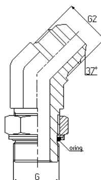
JIC 45 XWEP BSP / UNF
