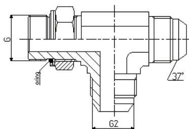
JIC XETP BSP / UNF
