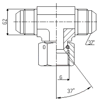
JIC XET UNF / UNF
